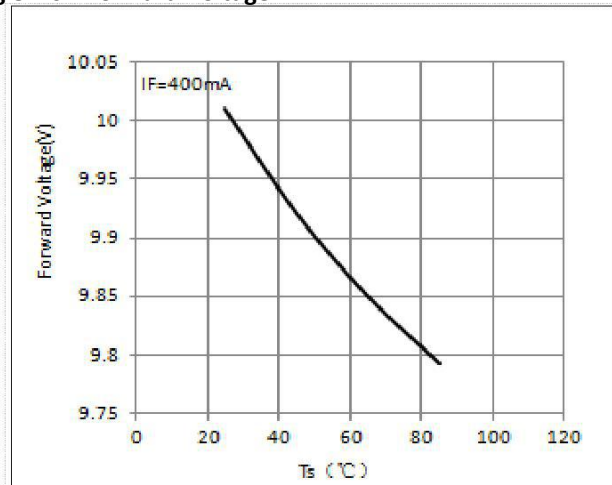
Fig 8. T_s —Forward Voltage.
